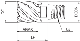
无内冷油孔, without Coolant Hole
