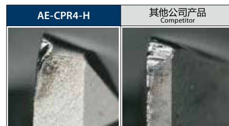
加工80.2m (型腔14个) 后的刃尖磨损情况 Wear condition of outer peripheral cutting edge after milling 80.2m
