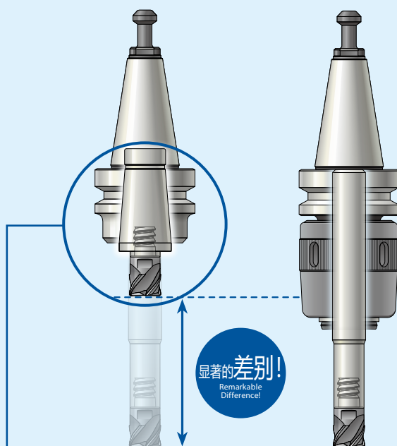
PXMC超短型 PXMC Collet Extra Short Type
