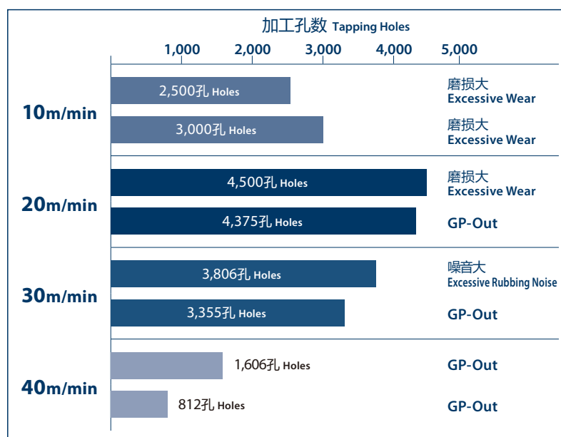
■不同的切削速度下耐久性对比 Comparison of durability by the difference in cutting speed
