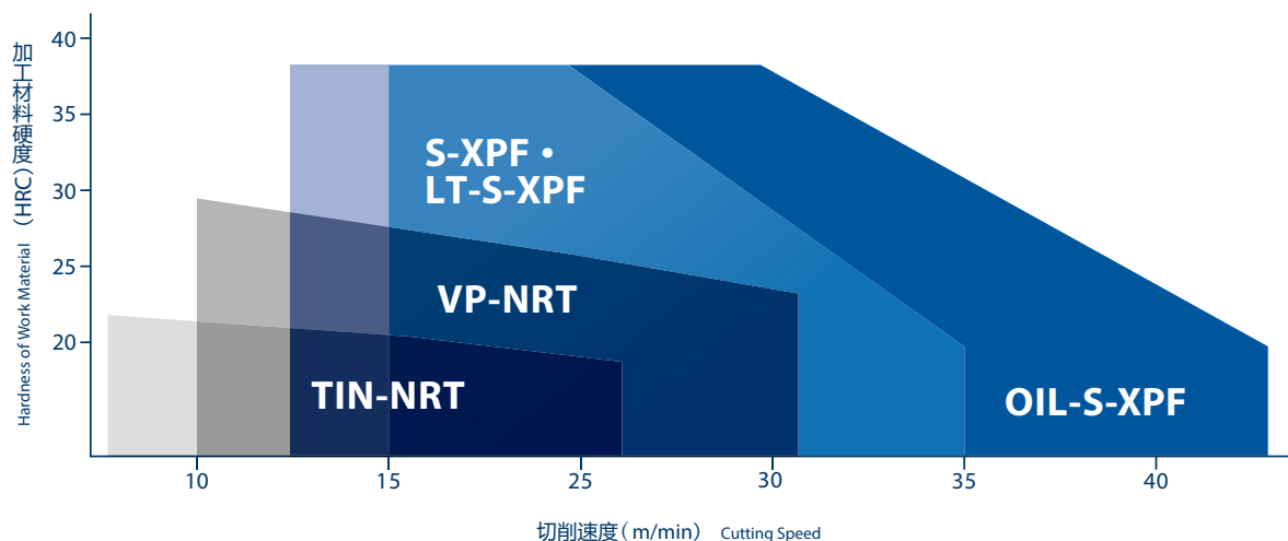
按硬度及切削速度区分的刀具选型图 Hardness and Cutting Speed Selection Image
